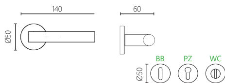
04 ROSETTE HANDLE
