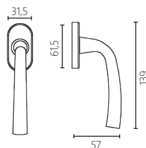
DK DRY KEEP WINDOW HANDLE
