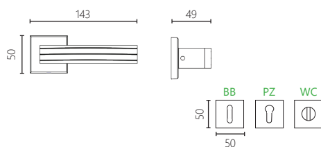
04 ROSETTE HANDLE
